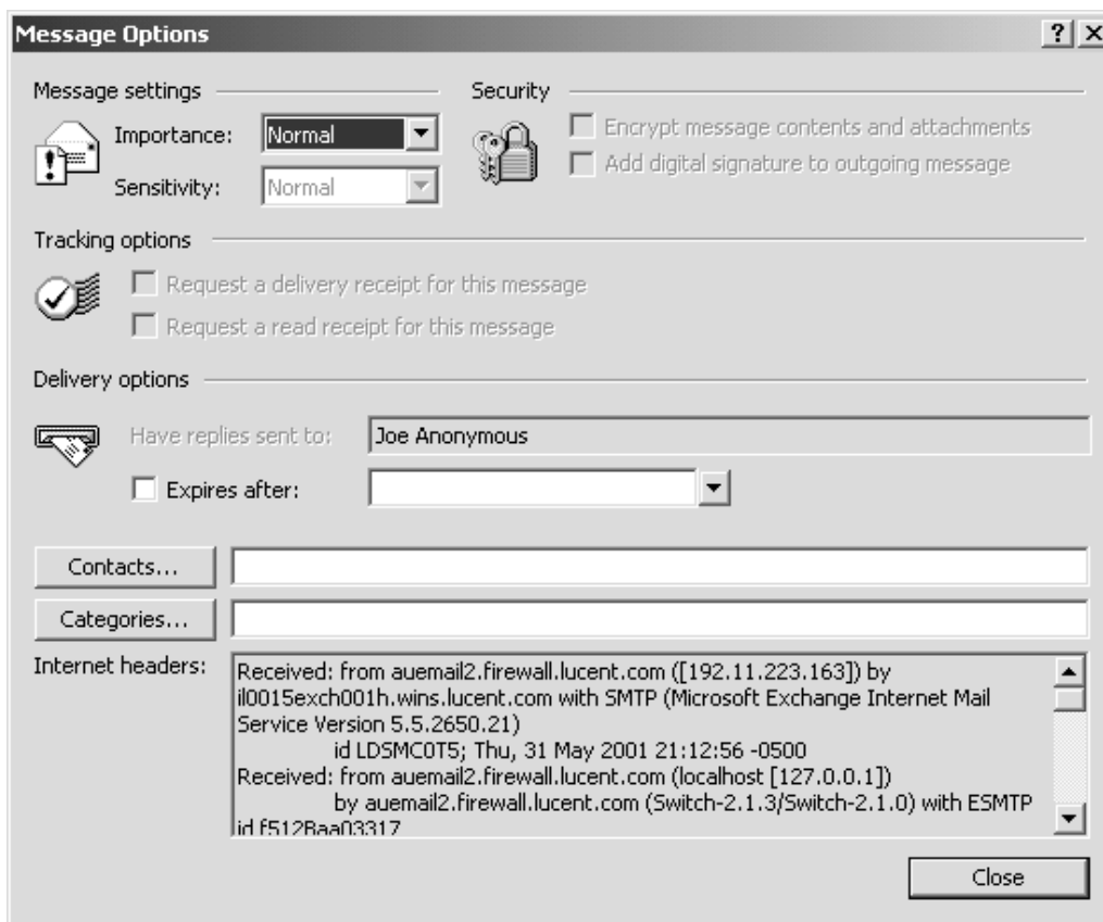
Figure 2-10 Viewing a message header in Microsoft Outlook
