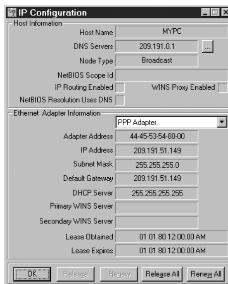
Figure 2-22 Extended winipcfg information
