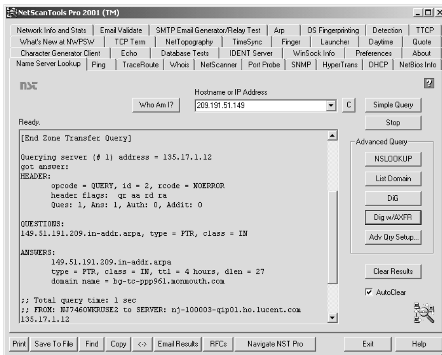
Figure 2-8 Using NetScanTools to investigate an IP address
